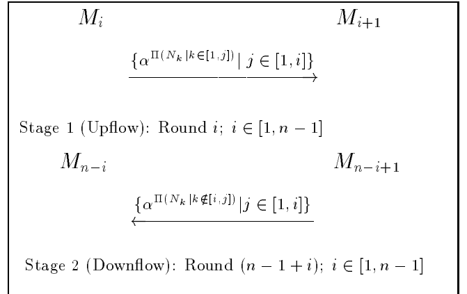
Figure 1: Group Key Distribution – GDH.1
